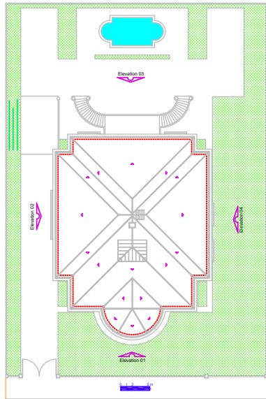
Roof Plan
