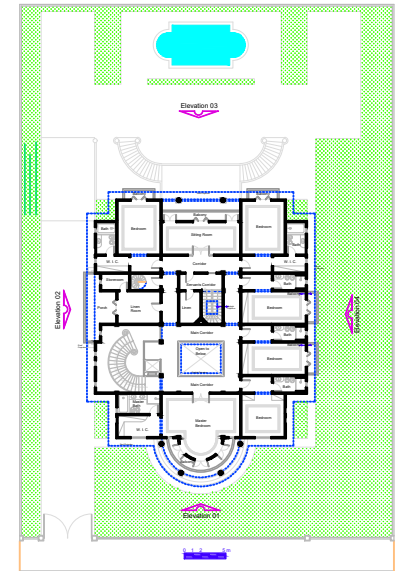
Second Floor Plan A = 392,72 m 2
