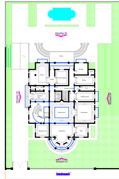
First Floor Plan A = 442,98 m 2
