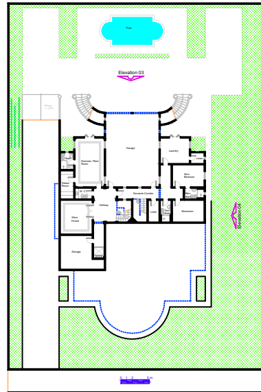
Lower Floor Plan A = 291,92 m 2
